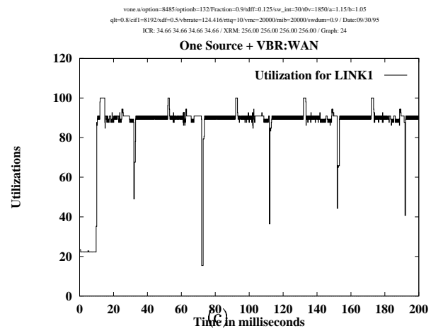
Figure 10: ERICA: One-source + VBR, WAN
