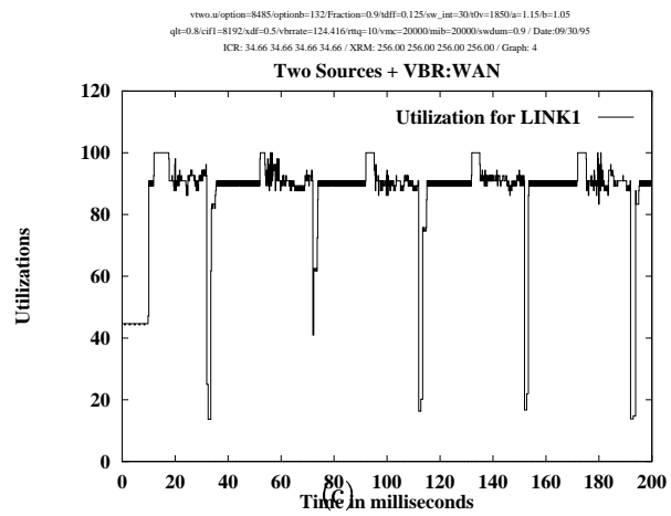
Figure 8: ERICA: Two-sources + VBR, WAN
