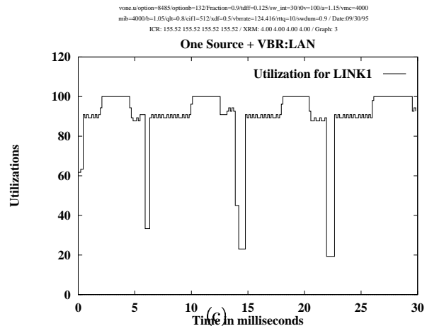
Figure 1: ERICA: One-source + VBR,LAN
