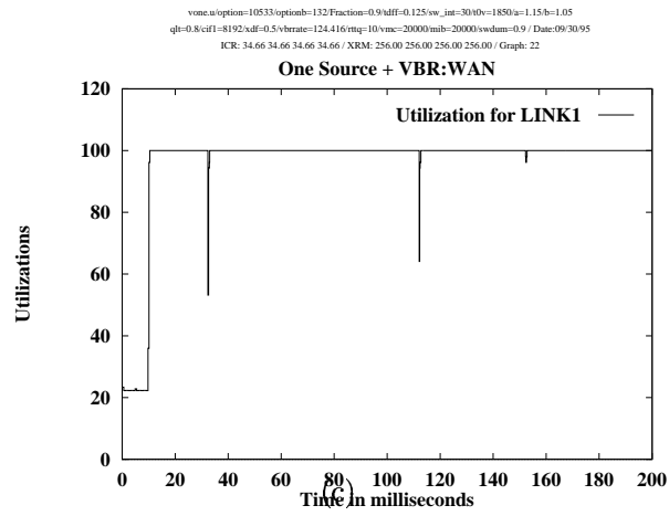
Figure 9: ERICA+: One-source + VBR, WAN
