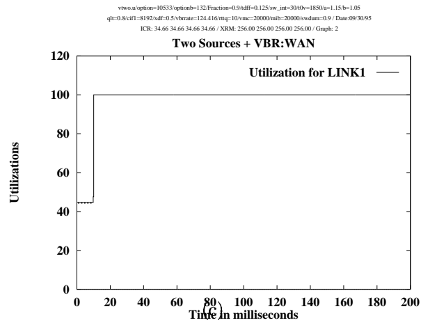
Figure 7: ERICA+: Two-sources + VBR, WAN
