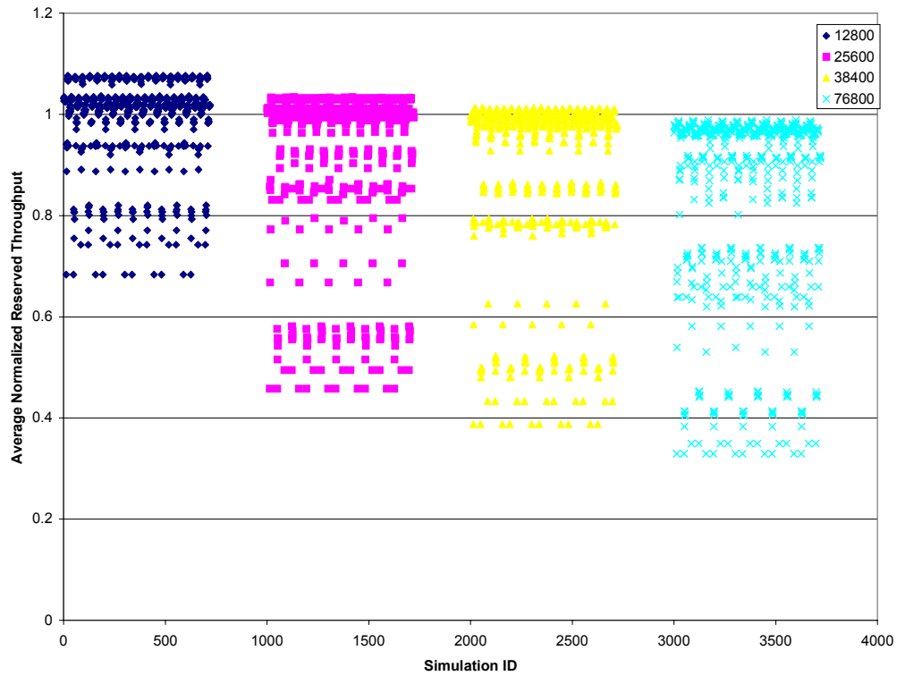
Figure 3 (c). Reserved Rate Utilization by TCP Customers in Three Color Simulations
