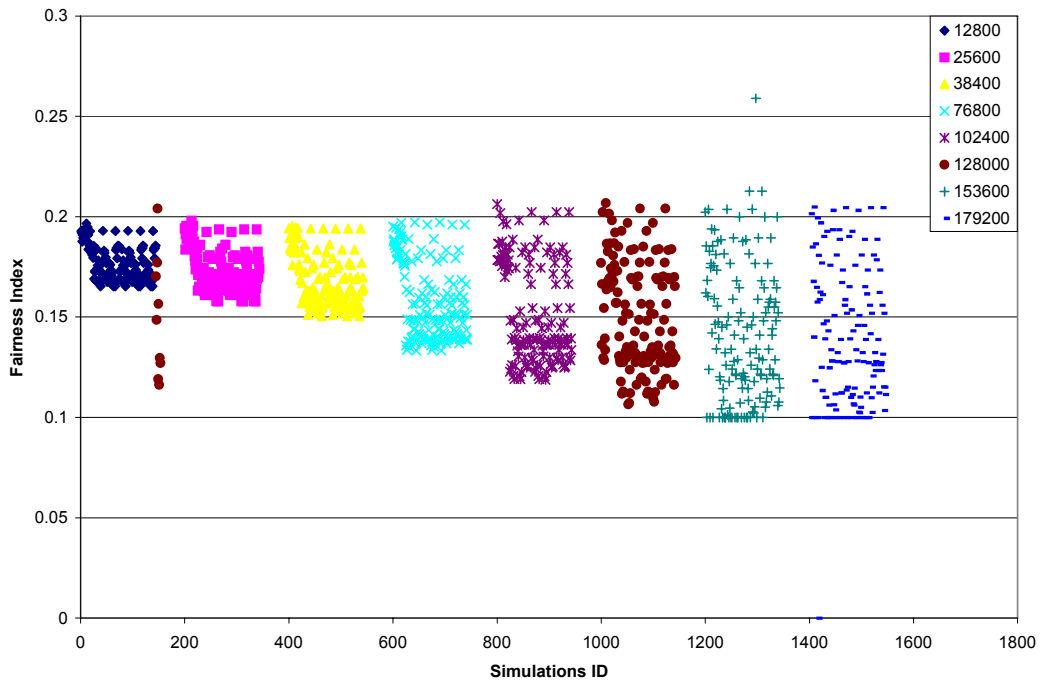
Figure 2 (a). Simulation Results: Fairness Achieved in Two Color Simulations with Different Reserved Rates
