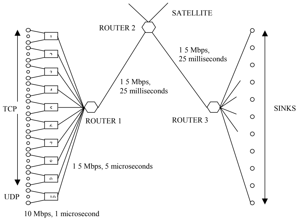
Figure 1. Simulation Configuration LEO
