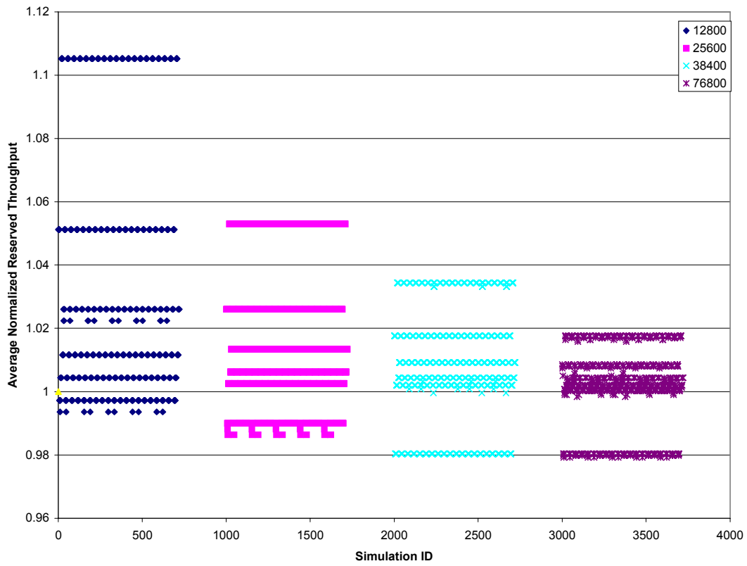
Figure 3 (d). Reserved Rate Utilization by UDP Customers in Three Color Simulations
