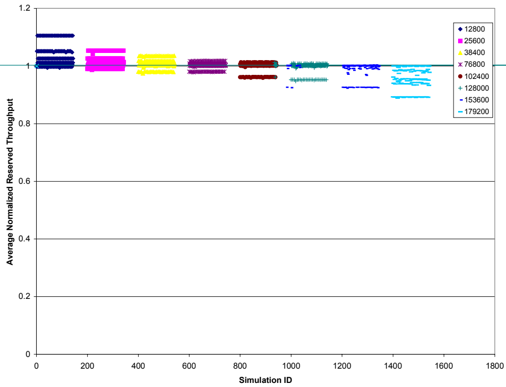
Figure 3 (b). Reserved Rate Utilization by UDP Customers in Two Color Simulations
