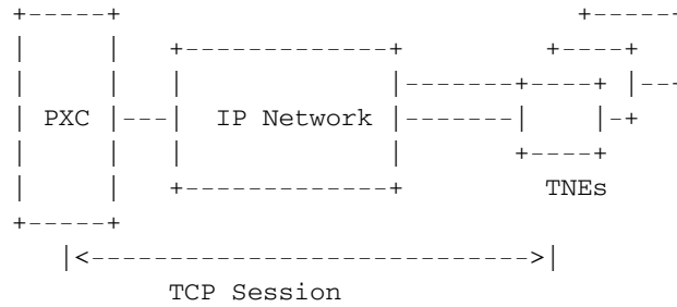
FIGURE 2: PXC-TNE Logical Connectivity
