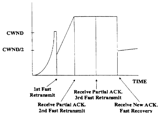
Fig. 6. TCP with the fast retransmit phase.
