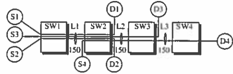
Fig. 3. Sample configuration for max-min fairness.
