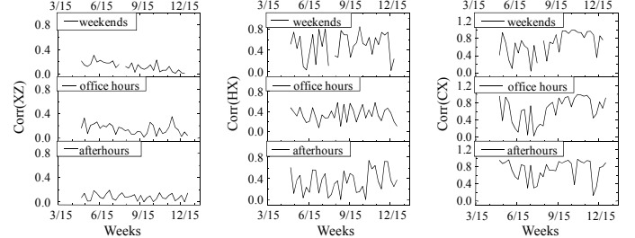
Fig. 14. Correlation comparisons among office hours, after hours, and weekends. The correlations are Corr(XZ), Corr(HX), and Corr(CX) from left to right respectively. (Z: electrical energy, H: heating, C: Cooling, X: temperature, Y: humidity).
