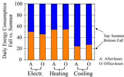
Fig. 17. The daily energy consumption comparison between Summer and Fall, considering after hours and office hours
