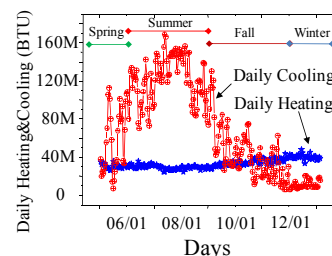
Fig. 8. Daily heating and cooling
