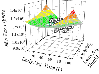
Fig. 10. Daily electrical energy consumption MPR regression plane
