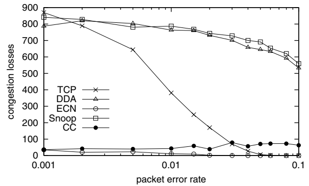
Figure 10. Congestion losses
