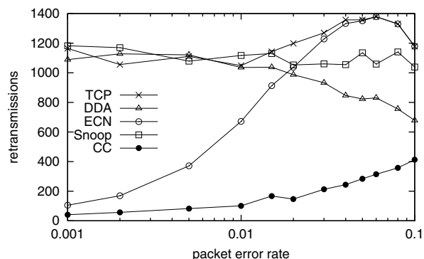
Figure 13. End-to-end retransmissions
