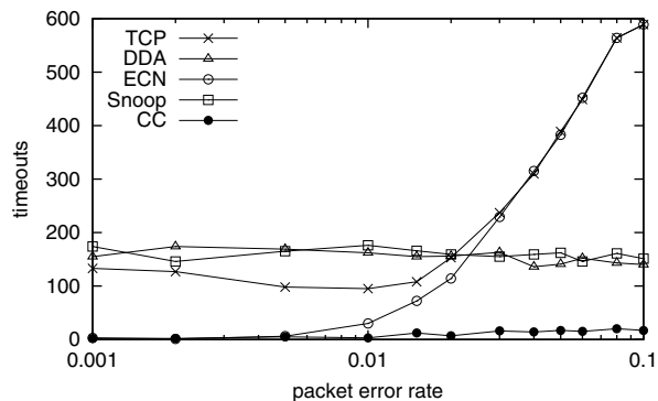
Figure 12. Number of timeouts
