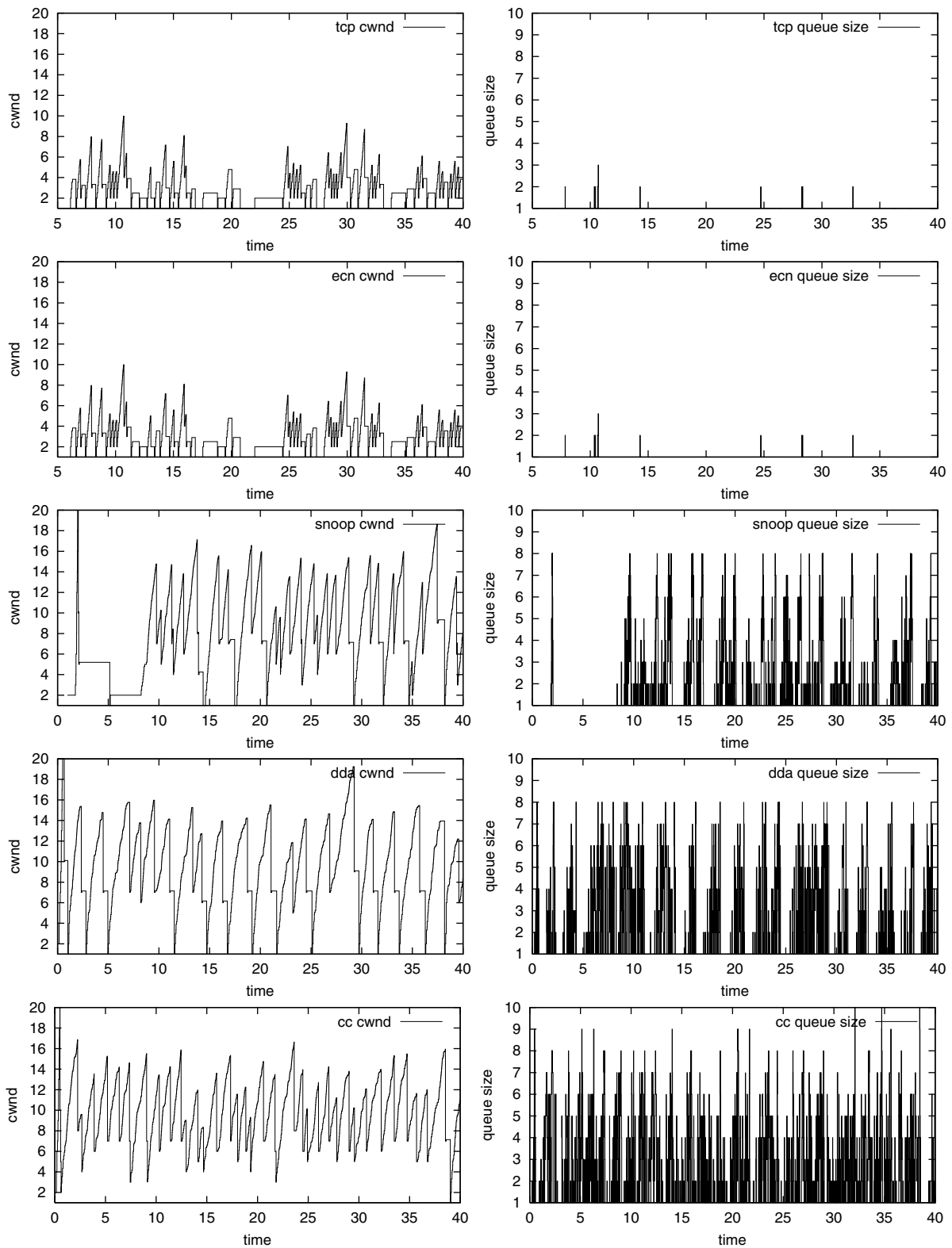
Figure 7. Congestion window and queue length for base TCP, ECN, Snoop, DDA and CC
