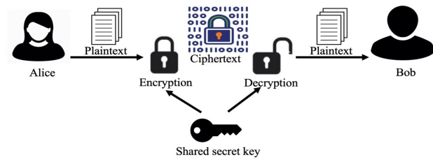
Fig. 4. Symmetric cryptography.
