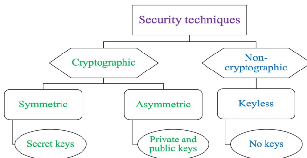
Fig. 3. Security techniques.
