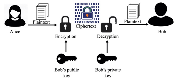
Fig. 5. Asymmetric cryptography.
