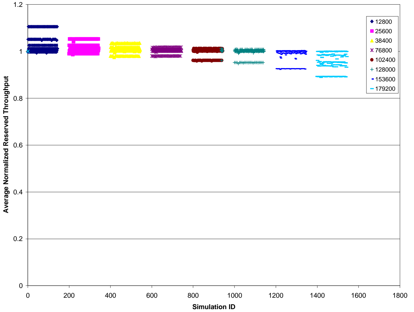
Figure 3 (b). LEO Reserved Rate Utilization by UDP Customers in Two Color Simulations
