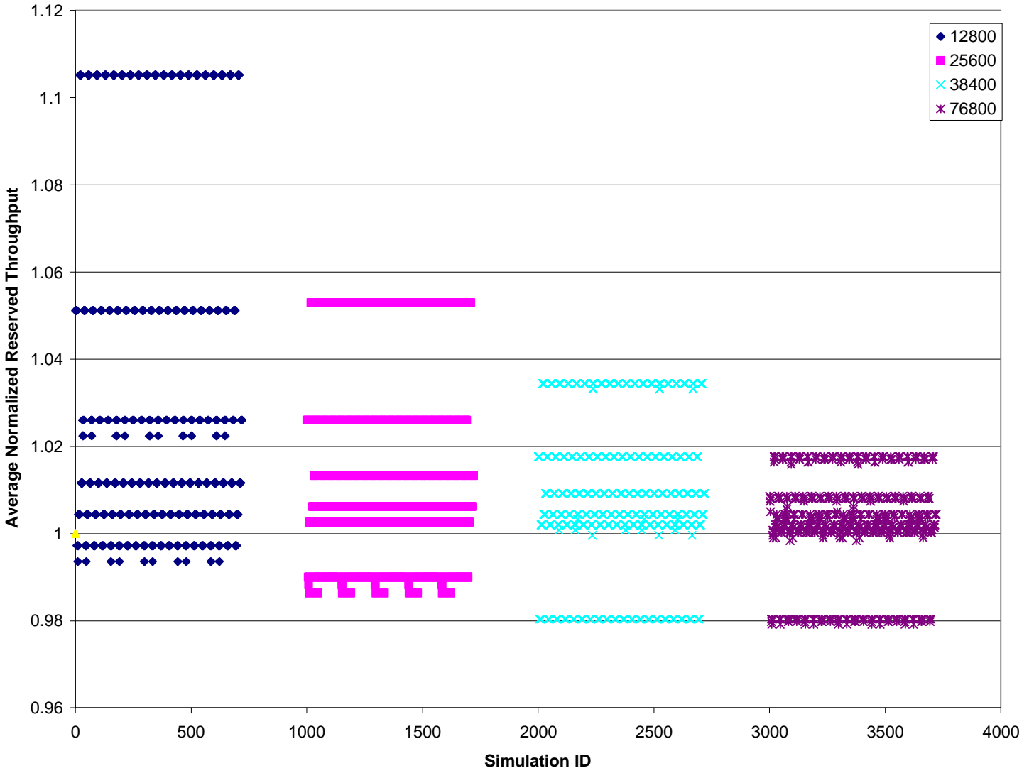
Figure 3 (d). LEO Reserved Rate Utilization by UTP Customers in Three Color Simulations
