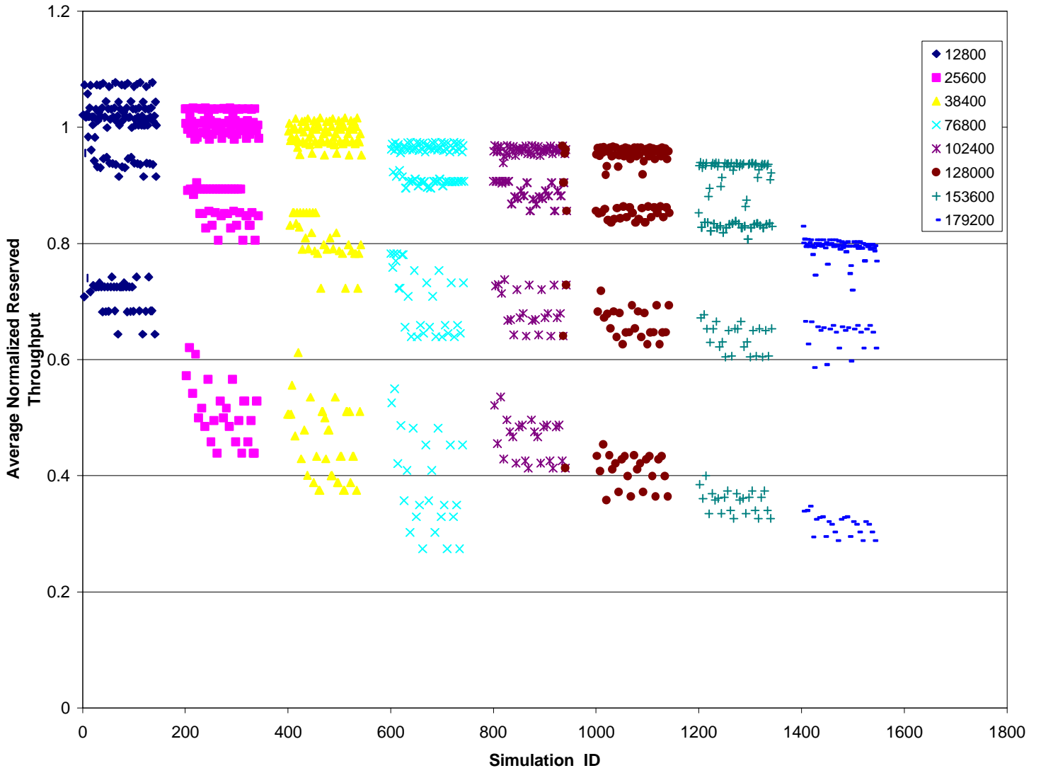
Figure 3 (a). LEO Reserved Rate Utilization by TCP Customers in Two Color Simulations
