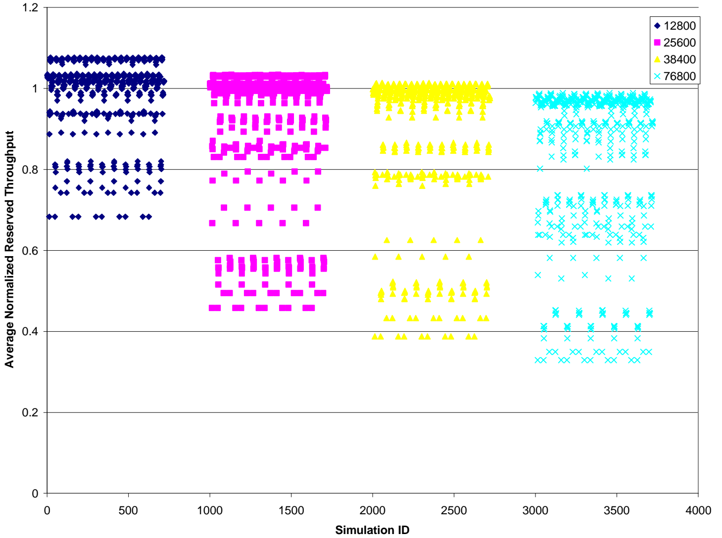
Figure 3 (c). LEO Reserved Rate Utilization by TCP Customers in Three Color Simulations
