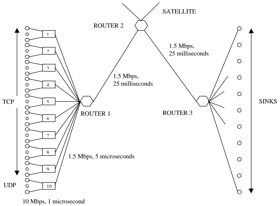
Figure 1. Simulation Configuration LEO
