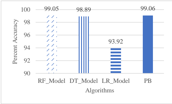
Fig. 4: Accuracy results of the first experimental setup
