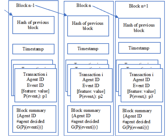
Fig. 2. The proposed transactions and blocks architecture
