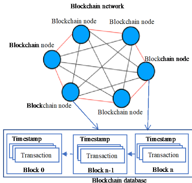
Fig. 1. Blockchain architecture
