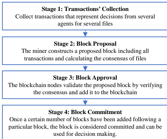
Fig. 3. The workflow for the proposed probabilistic blockchains
