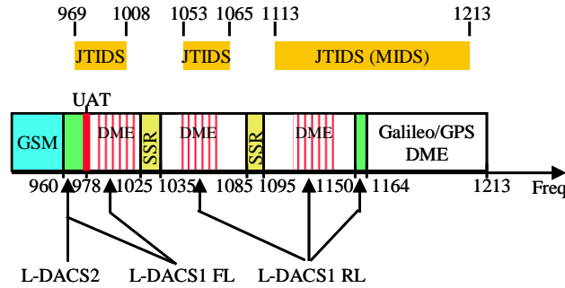
Figure 2: L-Band Spectrum Usage.
