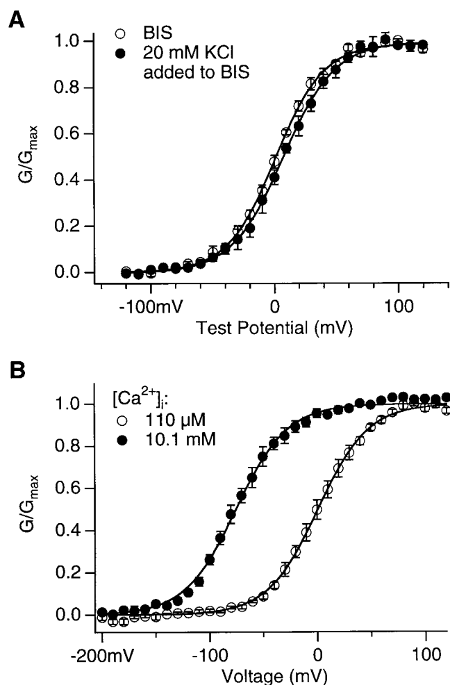
FIGURE 5. The effects of [KCl]_i and high [Ca^{2+}]_i on the activation of mslo1 channels. (A) G-V relations of mslo1 channels with or without 20 mM KCl added to the basal internal solution (BIS; MATERIALS AND METHODS). The total [Cl^-]_i is 22 mM and 2 mM, respectively. The total [K^+]_i is 162 and 142 mM, respectively. [Ca^{2+}]_i = 110 \mu M. The data was averaged from the results of n = 4 patches. Smooth lines are Boltzmann fits to data. With BIS, z = 1.29 and V_{1/2} = 1.1 mV. With 20 mM [KCl]_i added to BIS, z = 1.21 and V_{1/2} = 7.2 mV. (B) G-V relations of mslo1 channels at 110 \mu M or 10.1 mM [Ca^{2+}]_i . Smooth lines are Boltzmann fits to data. At 110 \mu M [Ca^{2+}]_i , z = 1.09 and V_{1/2} = 1.0 mV. At 10.1 mM [Ca^{2+}]_i , z = 1.06 and V_{1/2} = -75.1 mV.
