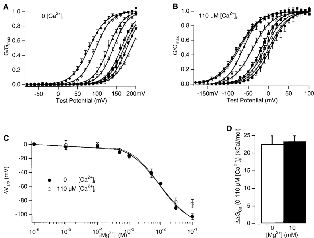
FIGURE 2. G-V relations in the presence of 0~100 mM [Mg^{2+}]_i at 0 (A) or 110 \mu M [Ca^{2+}]_i (B). The symbols represent [Mg^{2+}]_i at (in mM) 0 (open circle), 0.1 (closed circle), 0.5 (open square), 1 (closed square), 5 (open triangle), 10 (closed triangle), 30 (open diamond), and 100 (closed diamond). G-V relations from a number ( n ) of patches at each [Mg^{2+}]_i are averaged and plotted. Smooth curves are Boltzmann fits to averaged G-V relations. At 0 [Ca^{2+}]_i (A), z and V_{1/2} at various [Mg^{2+}]_i (mM) are as follows for 0, 1.17, 186.4 mV ( n = 12 ); for 0.1, 1.30, 177.0 mV ( n = 4 ); for 0.5, 1.26, 169.5 mV ( n = 4 ); for 1, 1.30, 162.7 ( n = 4 ); for 5, 1.36, 142.4 mV ( n = 4 ); for 10, 1.32, 129.6 mV ( n = 4 ); for 30, 1.30, 97.76 mV ( n = 7 ); and for 100, 1.13, 80.1 mV ( n = 8 ), respectively. At 110 \mu M [Ca^{2+}]_i (B), z and V_{1/2} at various [Mg^{2+}]_i (mM) are as follows: for 0, 1.10, 1.2 mV ( n = 10 ); for 0.1, 1.17, 5.8 mV ( n = 5 ); for 0.5, 1.12, -7.6 mV ( n = 6 ); for 1, 1.20, -16.0 ( n = 6 ); for 5, 1.06, -38.2 mV ( n = 5 ); for 10, 1.26, -62.5 mV ( n = 4 ); for 30, 0.97, -70.4 mV ( n = 4 ); and for 100, 0.95, -73.4 mV ( n = 4 ), respectively. (C) Left shifts of G-V relations on the voltage axis caused by various [Mg^{2+}]_i at 0 and 110 \mu M [Ca^{2+}]_i . \Delta V_{1/2} = (V_{1/2} at each [Mg^{2+}]_i - V_{1/2} at 0 [Mg^{2+}]_i ) obtained from n = 4 patches at 0 [Ca^{2+}]_i and n = 6 patches at 110 \mu M [Ca^{2+}]_i , are averaged and then plotted. The smooth curves are fits of Eq. 1 to data at 0 [Ca^{2+}]_i with z = 1.30 . For the thick curve, m is fixed at 4, K_C = 15.0 mM, K_O = 3.6 mM. For the thin curve, m is let free in the fit and is 1.94, K_C = 45.7 mM, K_O = 2.12 mM. (D) Changes in the activation energy provided by Ca^{2+} binding as the result of an increased [Ca^{2+}]_i from 0 to 110 \mu M in the absence or presence of 10 mM [Mg^{2+}]_i . -\Delta\Delta G_{Ca} = (zV_{1/2} at 0 [Ca^{2+}]_i - zV_{1/2} at 110 \mu M [Ca^{2+}]_i) eN , where e is elementary charge and N is Avogadro's number. Averaged from n = 4 patches.
